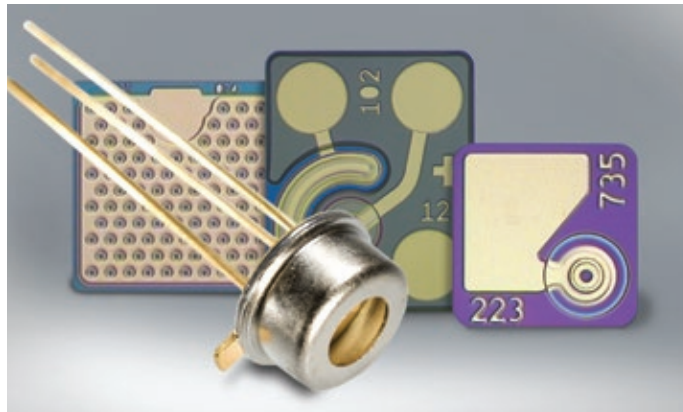
Clockwise from top: 850nm SM TO46; High-Power VCSEL Array; TBC VCSEL; 850nm SM Chip
